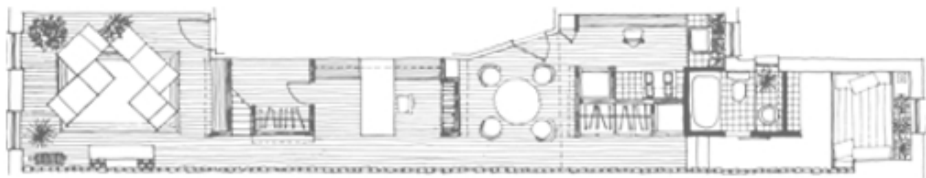
FLOOR PLAN
